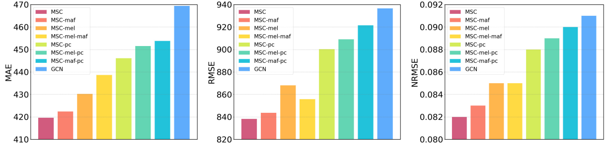
Figure 6: Ablation study with six variants of MSC across different metrics.
