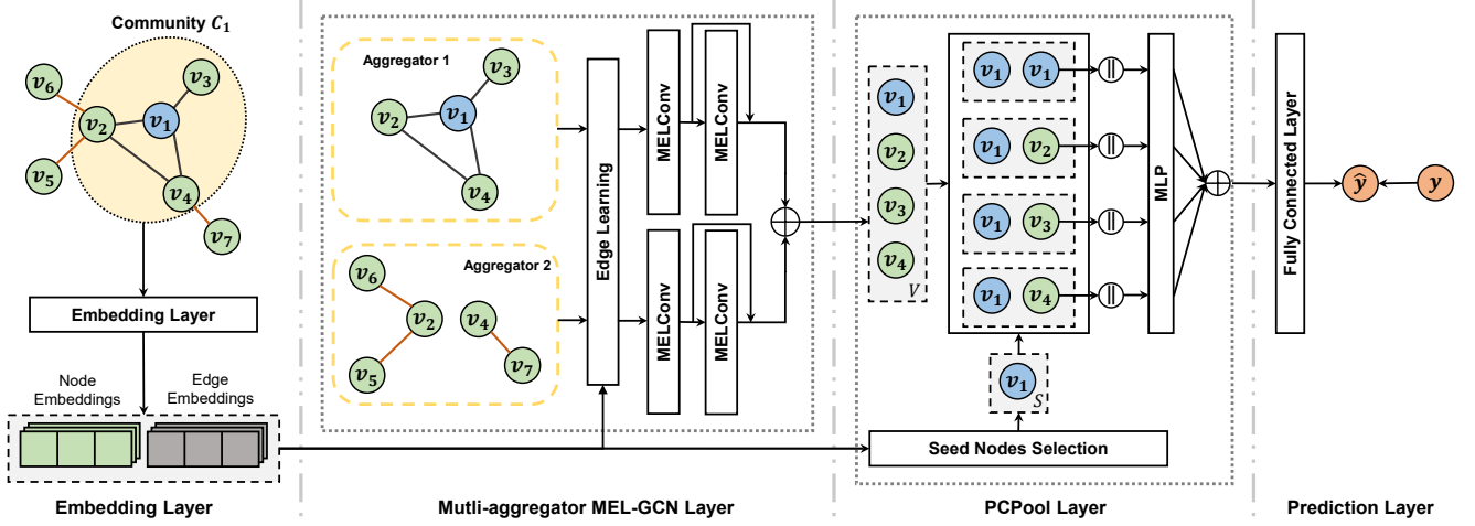
Figure 4: The architecture of our proposed Multi-scale Structure-aware Community Value Prediction Network (MSC). Here, we take the prediction of a demo community as an example. The multi-aggregator MEL-GCN layer takes the node embeddings, edge embeddings, and the adjacency matrix of community C_1 as inputs, and learns a node representation for each node by a masked edge learning graph convolutional network with different aggregators for intra-community edges and inter-community edges. The PCPool layer transforms the learned node representations to community representations for prediction through a pair-wise pooling mechanism controlled by the selected seed nodes that introduce prior knowledge.
