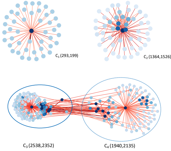
Figure 8: Case study of the edge learning weights of MEL-GCN, where the numbers in parentheses represent the prediction value and true value of the community.
