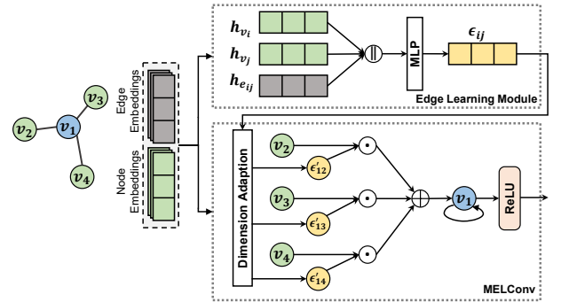
Figure 5: An illustration of the framework of MEL-GCN.
