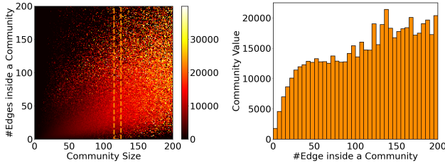
Figure 2: The correlation between community value and the number of edges inside a community. The right figure shows the details of the orange box area of the left figure. Note that the absence of data points causes the black part in the upper left of the left figure.
