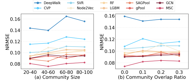
Figure 7: Performance comparison on datasets with different community sizes and different community overlap ratios.
