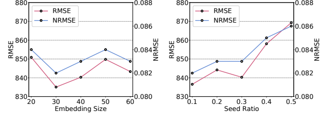
Figure 9: Hyper-parameter sensitivity analysis on the node embedding size and the seed ratio of PCPool.
