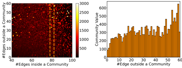
Figure 3: The correlation between community value and the number of edges outside a community. The right figure shows the details of the orange box area of the left figure.
