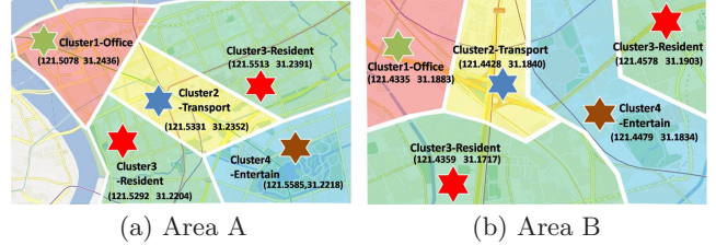
Figure 8: Two case studies for validating the geographical context of the five identified patterns.
